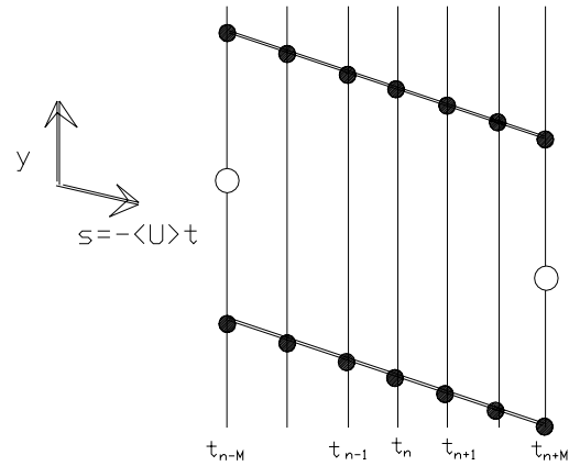
Figure 3. Diagram of the micro circulation domain used to calculate vorticity from the four wire probe.
