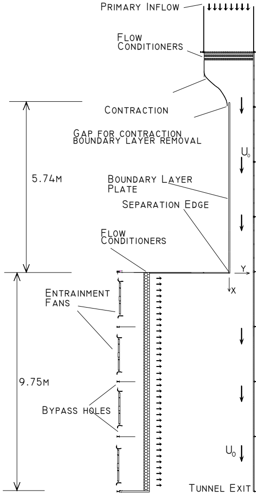
Figure 1. Schematic of the single stream shear layer facility.
