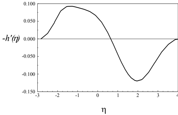
Figure 6. Reynolds stress gradient, obtained by fitting and differentiating the data shown in Fig. 5.
