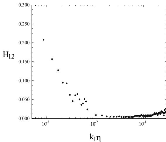
Figure 4. Coherence function: E_{12}^2 / E_{11}E_{22}
