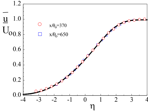
Figure 4. Mean velocity profile in the shear layer
