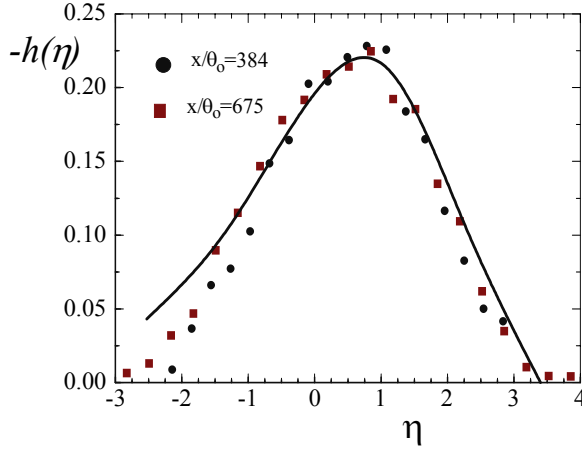
Figure 5. Calculated and measured Reynolds shear stress
