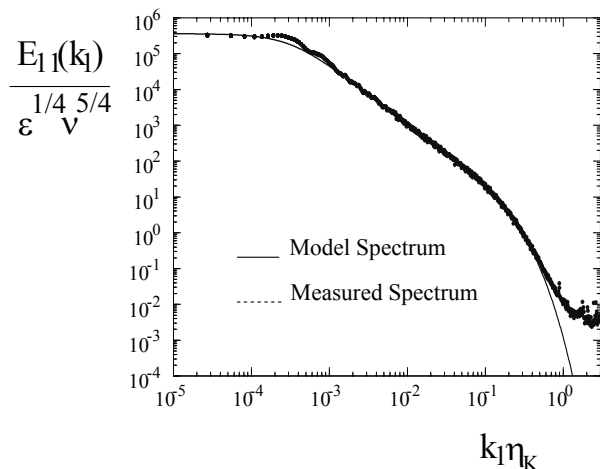
Figure 5. Power Spectral density E_{11} with model fit from Pope (2000).
